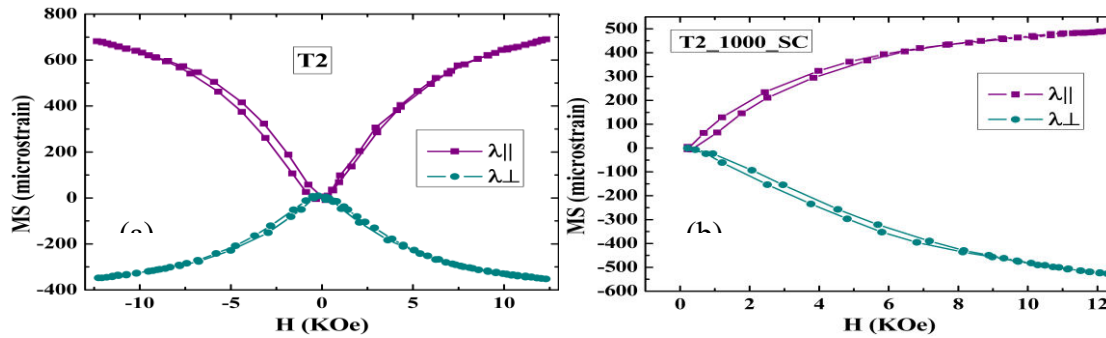
Figure 3: Room temperature MS values of (a) T2 and (b) T2_1000_SC alloys in parallel and perpendicular direction
