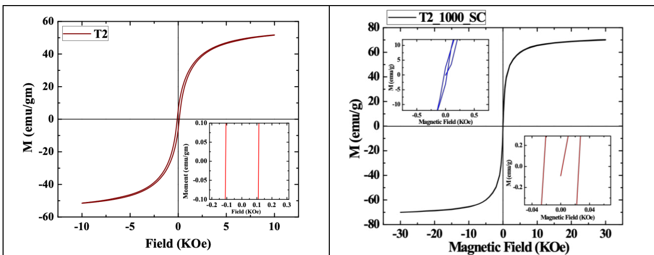
Figure 4: Room temperature M-H curves of (a) T2 and (b) T2_1000_SC samples.
