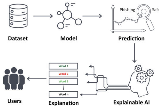
Figure 2: Overview of an Explainable Transformer-based Model (Uddin et. al., 2024)
