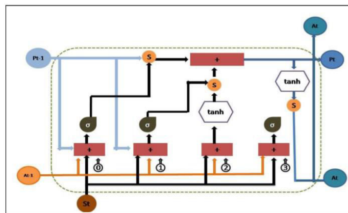
Fig. 3: Working of LSTM
