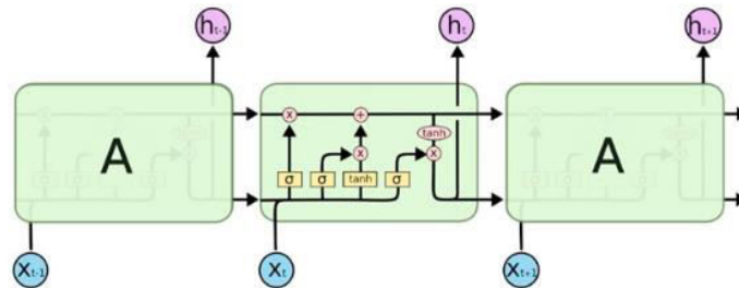
Fig. 1: The internal structure of an LSTM
