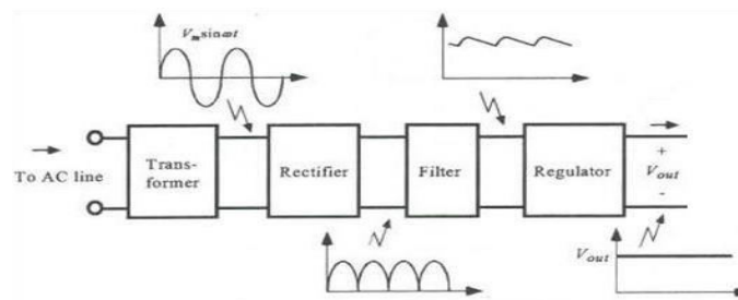
Fig:5.3(Block diagram of power supply)
