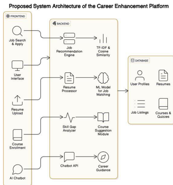
Fig. 1. System Architecture of Career Enhancement Platform
