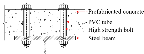
Fig. 11. Through bolts tested by Chen et al. [14]
