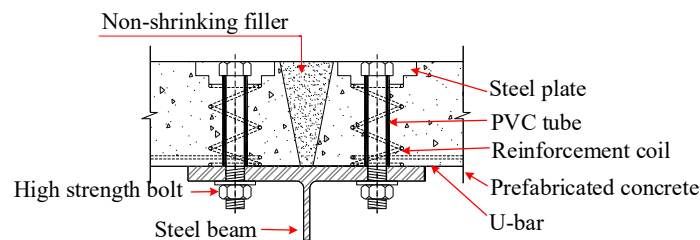
Fig. 10. The Krupp-Montex system [13]
