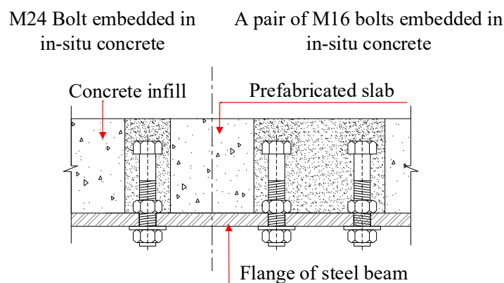
Fig. 5. Demountable shear connectors tested by Pavlovic [7]
