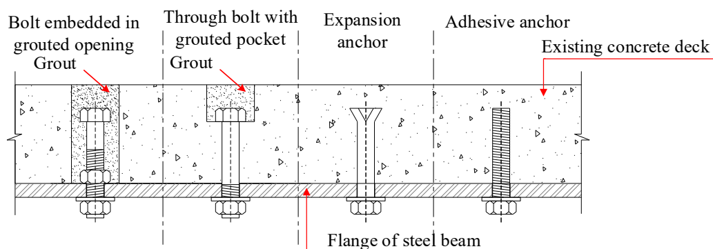
Fig. 4. Post-installed demountable shear connectors tested by Schaap [3] and Kwon et al. [4]
