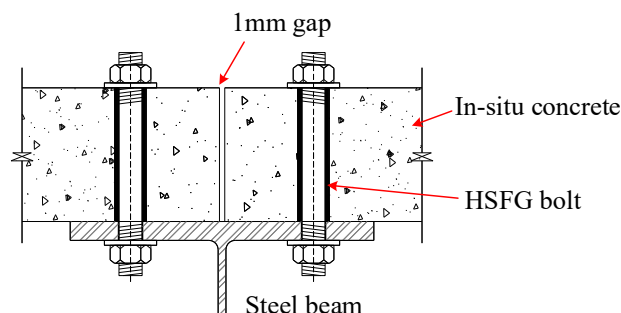
Fig. 8. Friction connection tested by Roik and Bürkner [11]
