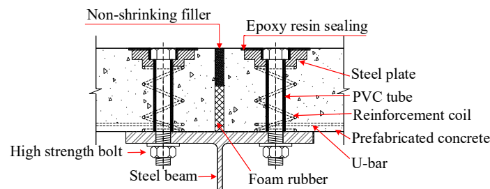
Fig. 9. Demountable shear connection for car parks proposed by [12]
