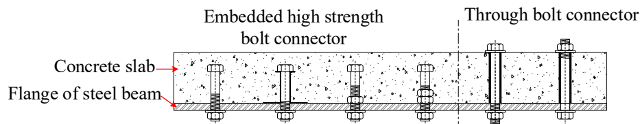
Fig. 1. Typical Construction Form of High-Strength Bolted Shear Connector for Steel-Concrete Composite Beams
