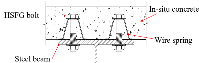
Fig. 2. High-strength friction grip bolts tested by Dallam[1]
