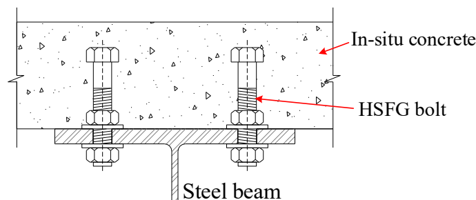
Fig. 6. Demountable shear connectors tested by Moynihan and Allwood [8]
