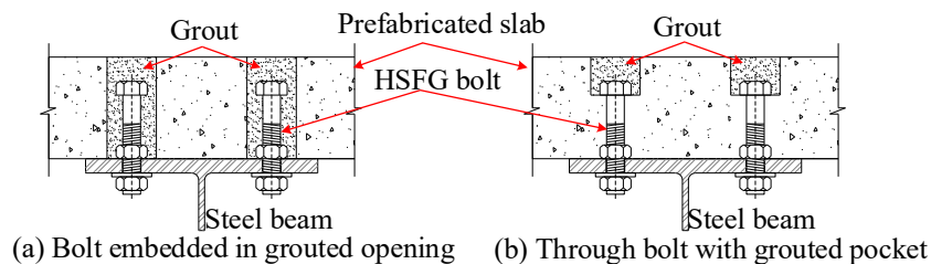
Fig. 3. Bolted shear connectors tested by Dedic and Klaiber [2]
