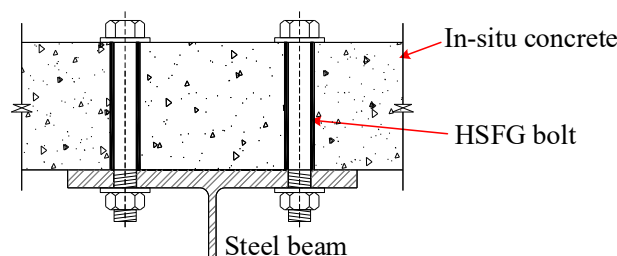
Fig. 7. Bolted shear connection tested by Marshall [10]
